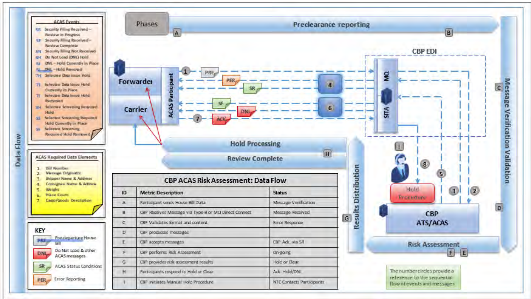
Figure 1. ACAS Processing Flow Reference Chart
